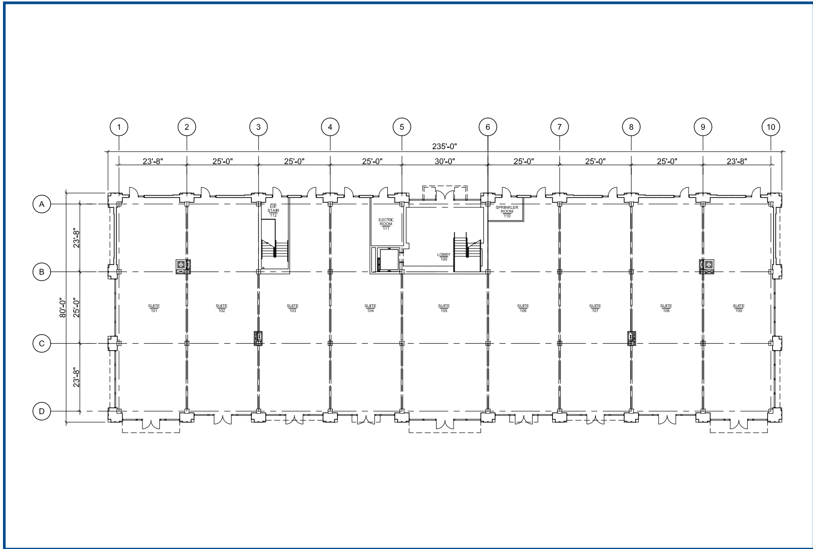
BUILDING THREE – 1ST LEVEL FLOORPLAN
