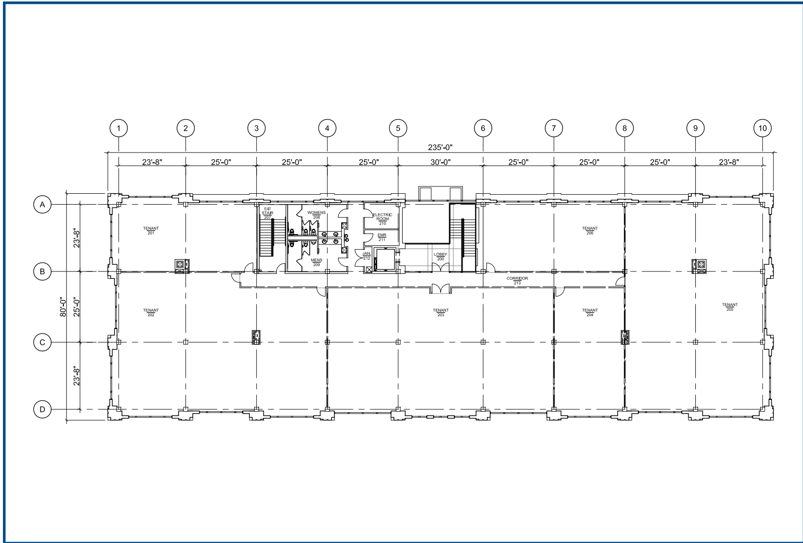
BUILDING THREE – 2ND LEVEL FLOORPLAN
