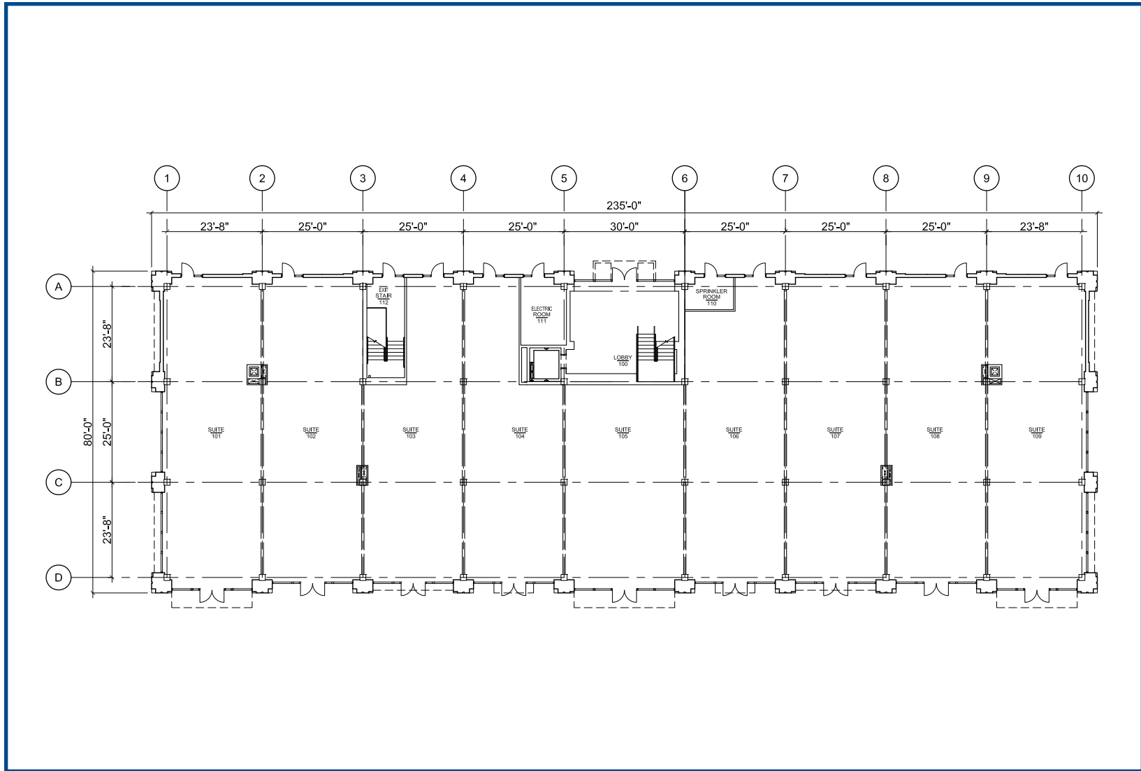
BUILDING TWO - 1ST LEVEL FLOORPLAN
