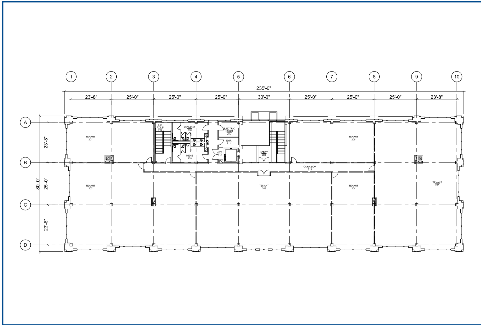
BUILDING TWO - 2ND LEVEL FLOORPLAN
